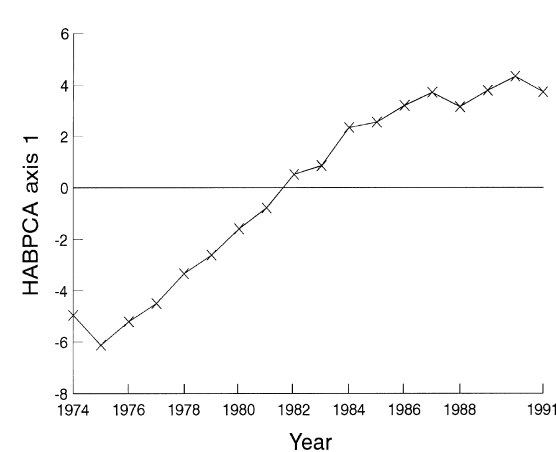
Fig. 3. Annual scores from the first axis of principal components analysis of agricultural variables, considering the 18 most accurately measured variables (Table 5).
