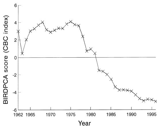
Fig. 4. Annual scores from the first axis of Principal components analysis of Common Bird Census index of 29 farmland bird species.
